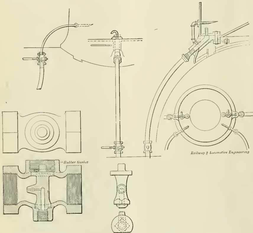
PNEUMATIC SANDING DEVICE, C. & N. W. RY.
